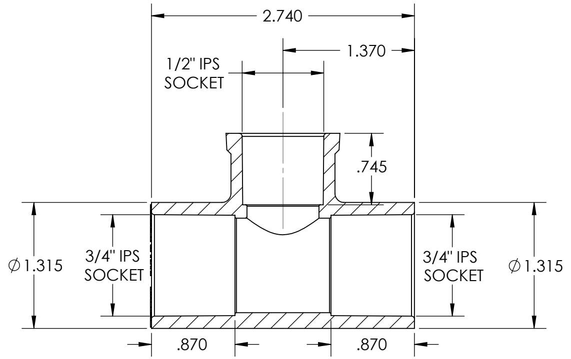
SECTION E-E
