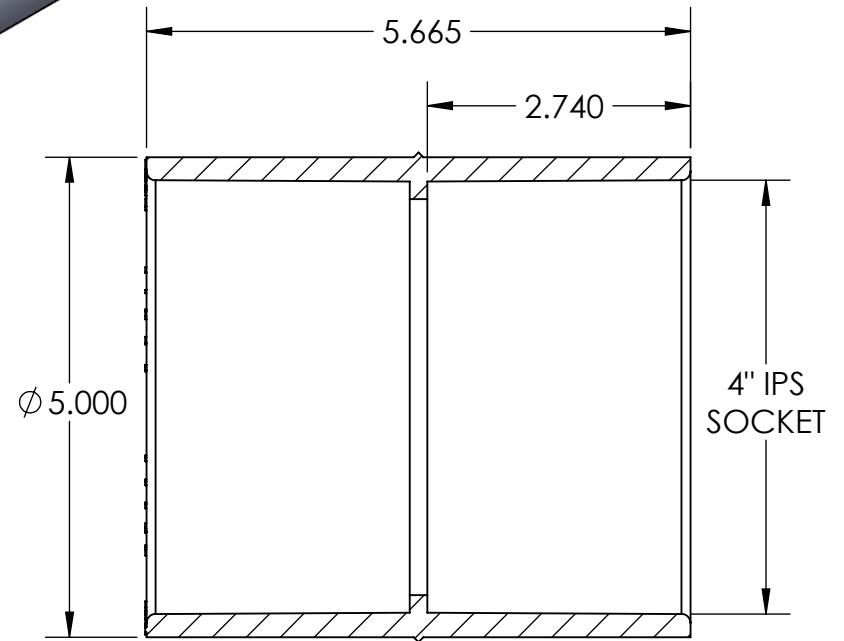
SECTION E-E
